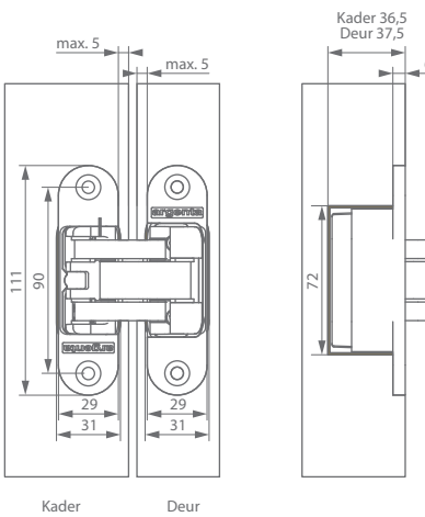
invisible medium brandwerend
