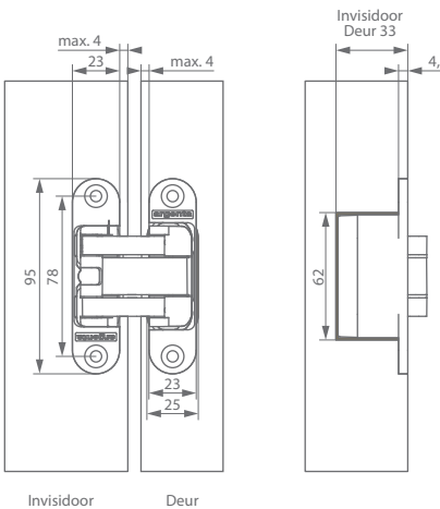
invisible small brandwerend
