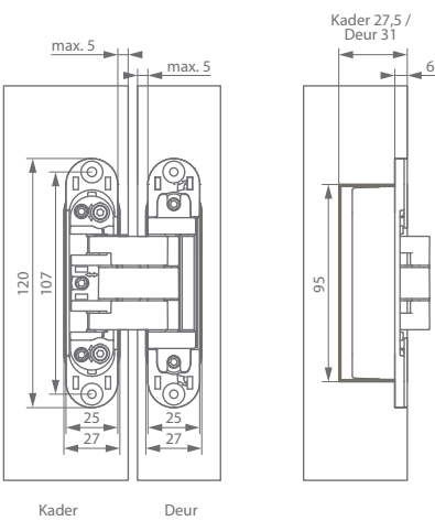
invisible neo M-6 brandwerend
